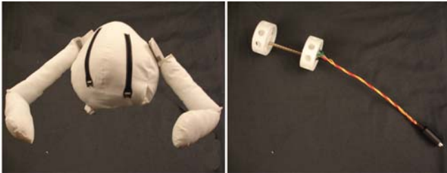
Fig. 3. TUI3D; Uniball interface; various limbs with own sensors, like the one to the right, can be plugged into a central interface (left) to control different skeleton structures.
